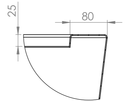
DETAIL 2 SCALE 1 : 5
