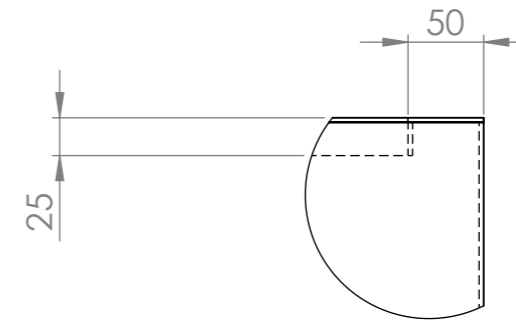
DETAIL A SCALE 1 : 5
