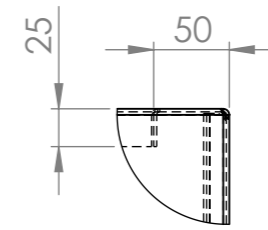
DETAIL A SCALE 1 : 5
