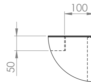
DETAIL C SCALE 2 : 15
