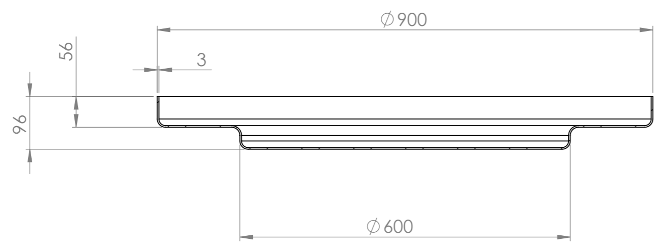
SECTION C-C
