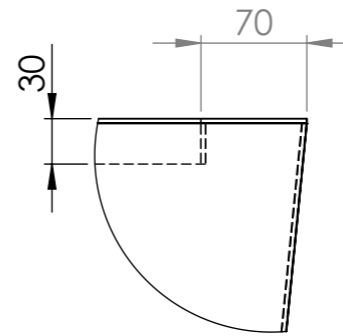
DETAIL C SCALE 1 : 5
