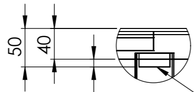
DETAIL B SCALE 1 : 5 Overflow
