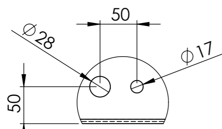
DETAIL C SCALE 1 : 5
