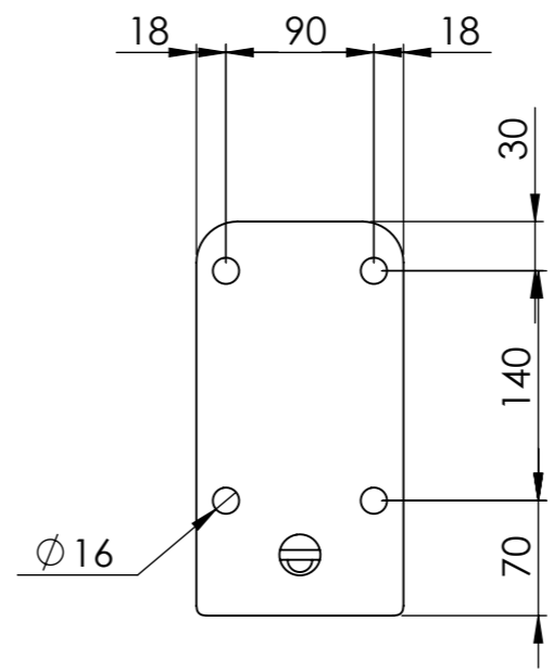
DETAIL G SCALE 1 : 5
