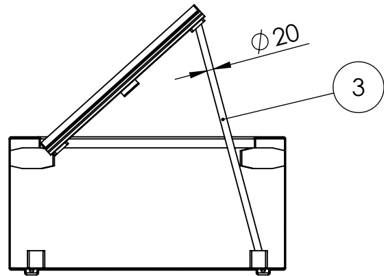
SECTION J-J
